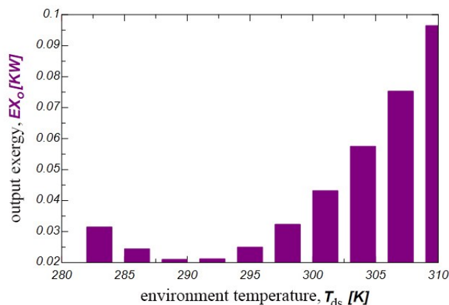
Fig. 8 The M-cycle output exergy rate
