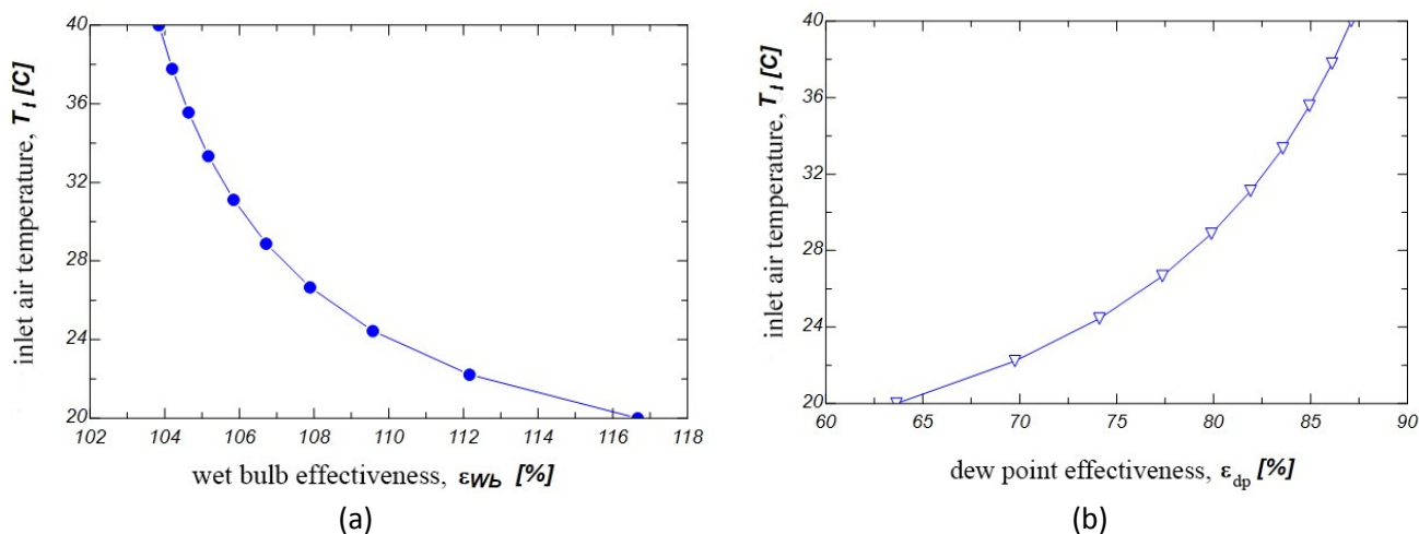
Fig. 4 (a) variations of the wet bulb effectiveness at different exchanger inlet air temperatures and (b) variations of the dew point effectiveness at different exchanger inlet air temperatures
