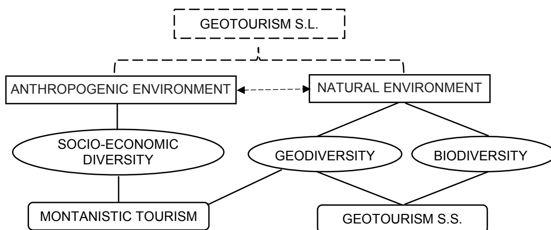
Fig. 3 Position of montanistic and geoscience tourism in diversity system
