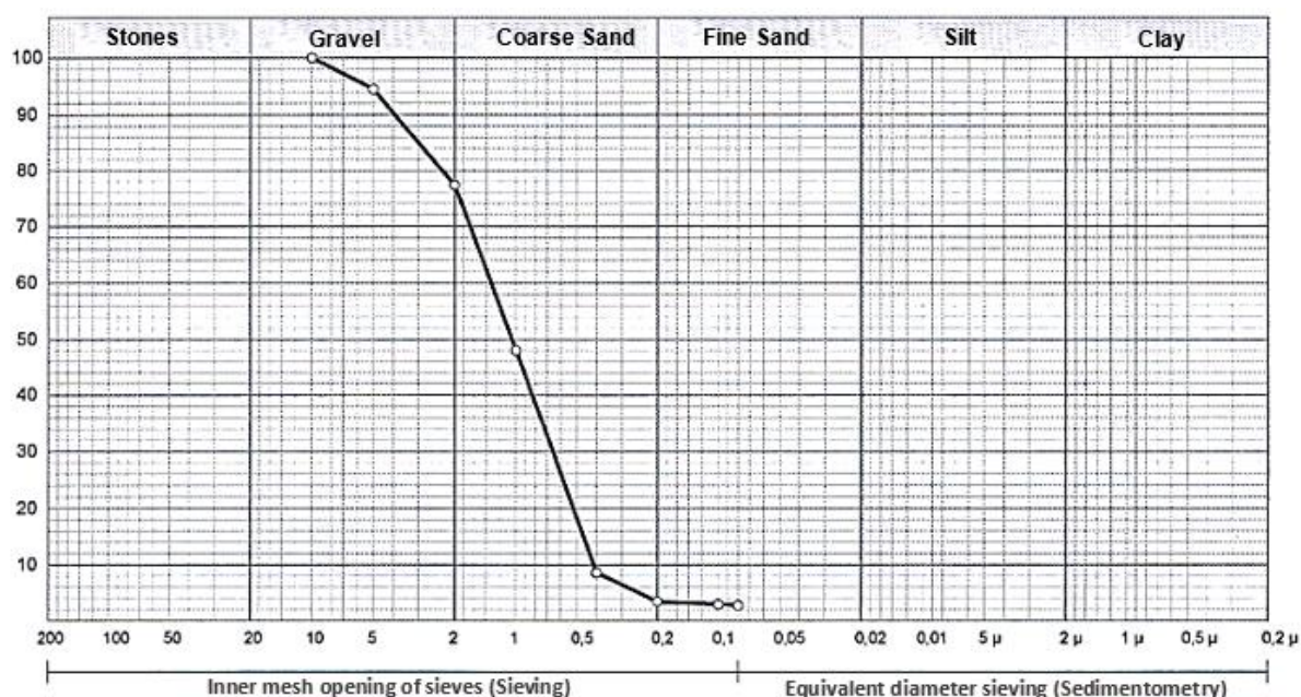
Figure 15. Grading curve of the sample taken along the upstream section of the Oued Fodda dam
