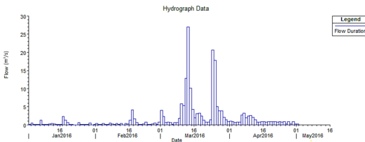
Figure 13. Flow hydrograph
