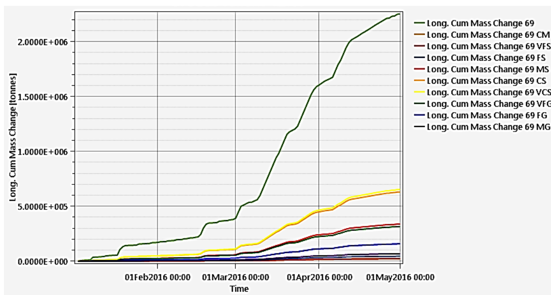
Figure 22. Sediment mass accumulation as a function of time at section 69 (downstream)
