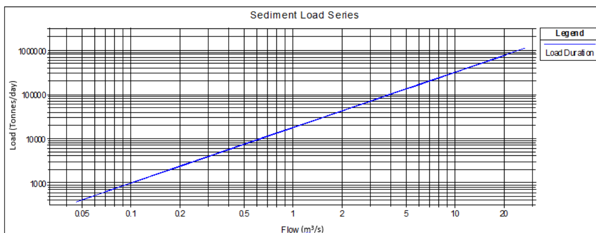
Figure 20. Sediment specific load curve
