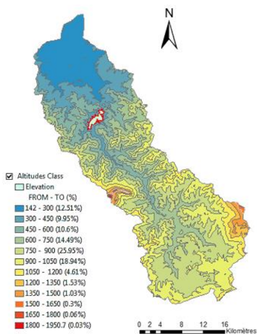
Figure 2. Hypsometric Oued Fodda watershed map
