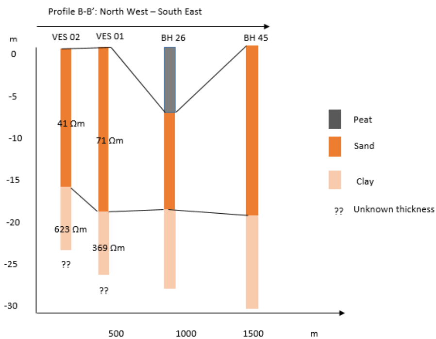
Fig. 6: Profiles of the subsurface lithology for profile BB I
