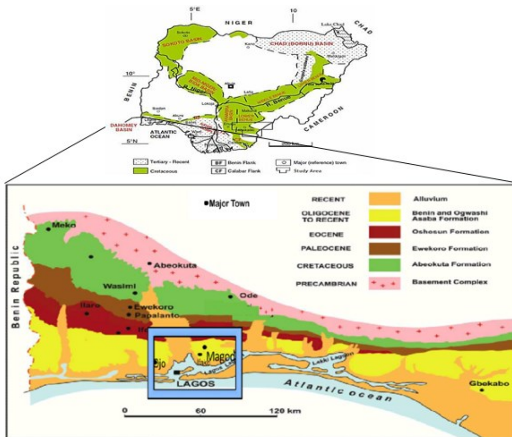
Fig. 2: Map of sedimentary basin of Nigeria showing the study area [15]; Inset: Geological Map of Dahomey basin showing the study area (modified according to [14])
