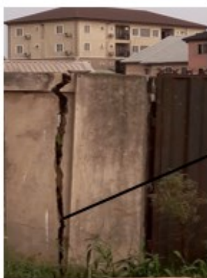
Fig. 1: Evidence of Structural Failure of Buildings in the Study Area
