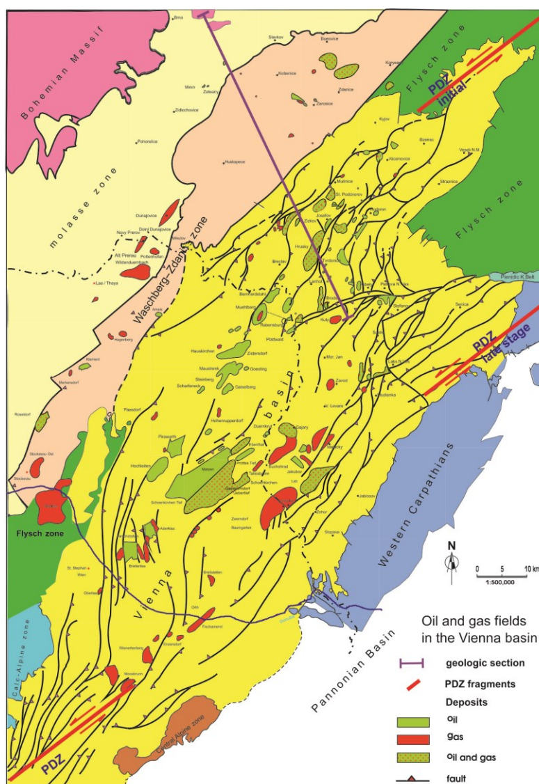
Fig. 1 Oil and gas fields in the Vienna basin (modified after Arzmüller et al., 2006; fragments of principal displacement zone PDZ are from Wu et al., 2009)
