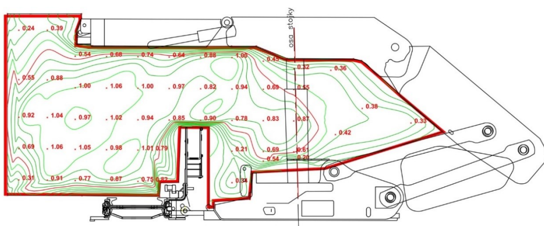
Figure 2 Speed profile of the measured velocity of air in a coalface with MEOS 25/56 support
